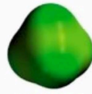
electrostatic potential
