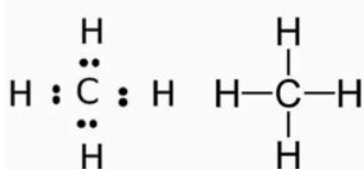
dot structure
