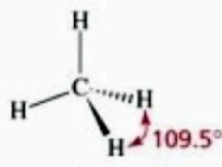
perspective formula
